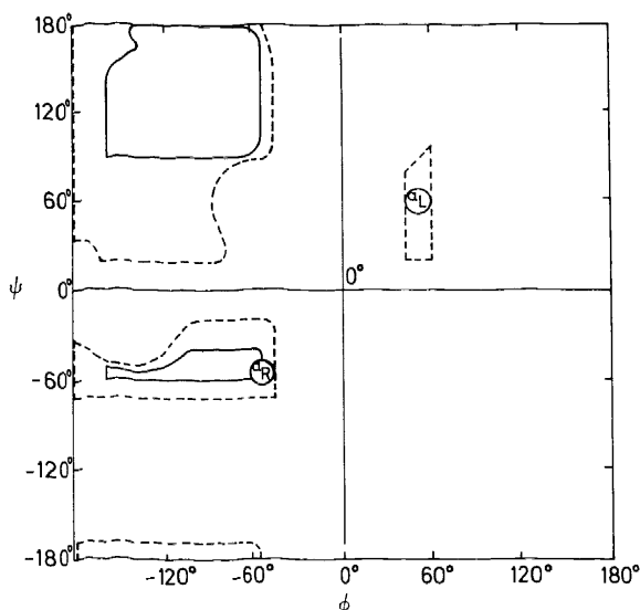
Figure 6. Typical conformational map (Ramachandran et al. 16 ) transposed into the standard conventions. Note: this diagram is identical with that of Edsall et al. 1 except that the origin is now at the center, instead of at the lower left-hand corner. The solid lines enclose the freely allowed values of \phi and \psi for an alanyl residue in a polypeptide; the dotted lines enclose 'outer limit' values based on the shortest known van der Waals radii in related structures. Analogous diagrams for other residues, and for slightly different assumptions, are given by Ramachandran and Sasisekharan 13 (note that these authors used the earlier convention with the origin at the corner).
