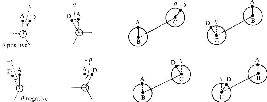
Figure 1. Newman and perspective projections illustrating positive and negative torsion angles. Note that a right-handed turn of the bond to the front atom about the central bond gives a positive value of \theta from whichever end the system is viewed.
