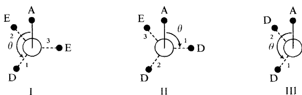
Figure 2. Tetrahedral configurations: case I, D > E = E ; case II, D = D > E ; III, D = D (E non-existent).
