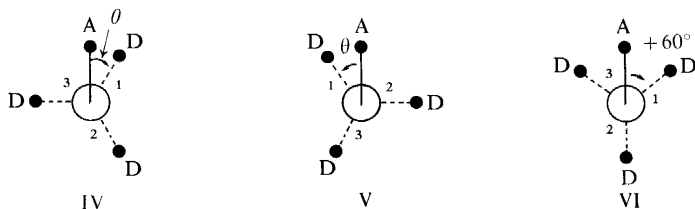
Figure 3. Tetrahedral configurations. Three identical branches: IV, general case, \theta positive; V, general case, \theta negative; VI, \theta = 60^\circ .
