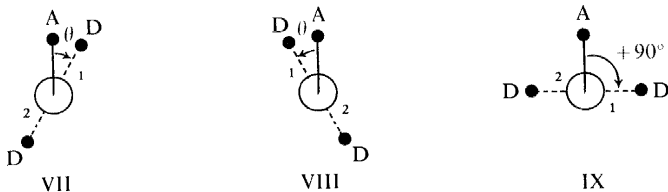
Figure 4. Planar trigonal configurations. Identical branches: VII, \theta positive; VIII, \theta negative; IX, \theta = 90^\circ .
