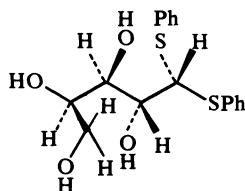
D-Ribose Diphenyl Dithioacetal: Conformation in CD_3OD-C_3D_5N
