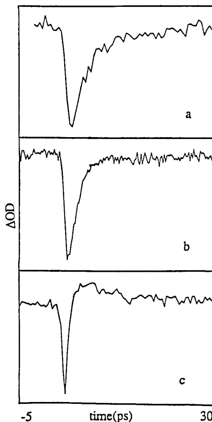
Figure 4. Absorption transients for betaine30 in acetone; \lambda_{\text{pump}}=800\text{nm} , \lambda_{\text{probe}}= a) 800nm, b) 700nm and c) 640nm
