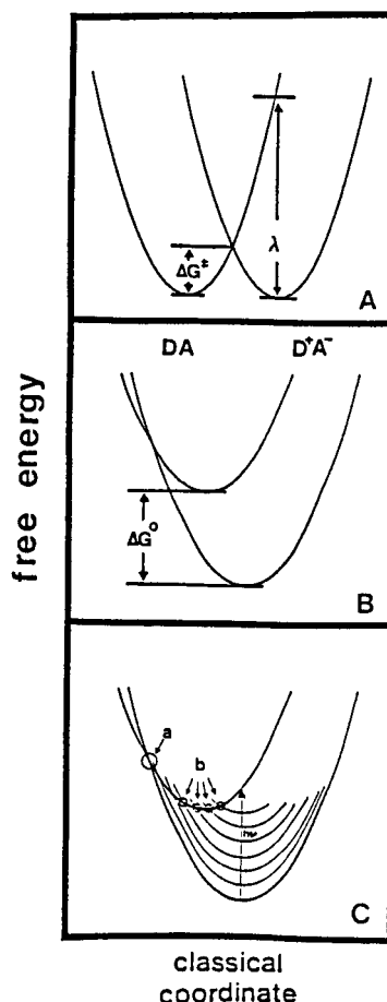
Figure 1. Surfaces representing the localization of the transferring electron donor (DA) and acceptor ( D^+A^- ). The classical reorganization energy is \lambda , the reaction free energy is \Delta G^\circ , the classical barrier to the reaction is \Delta G^\ddagger . A) \Delta G^\circ=0 . B) \Delta G^\circ + \lambda < 0 . C) same as B) with quantized vibrational mode in D^+A^- .
