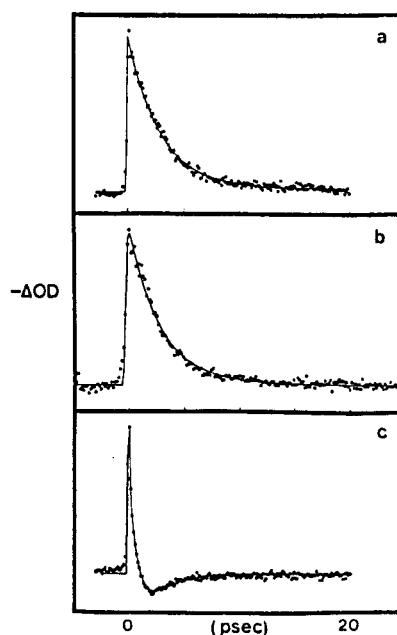
Figure 3. Absorption transients for betaine30 in a) toluene, b) benzene and c) acetone. Points are data, lines are biexponential fits to the data.
