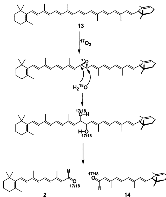
Fig. 9 Enzymatic cleavage of \alpha -carotene 13 in the presence of ^{17}\text{O}_2 and \text{H}_2\text{}^{18}\text{O} .
