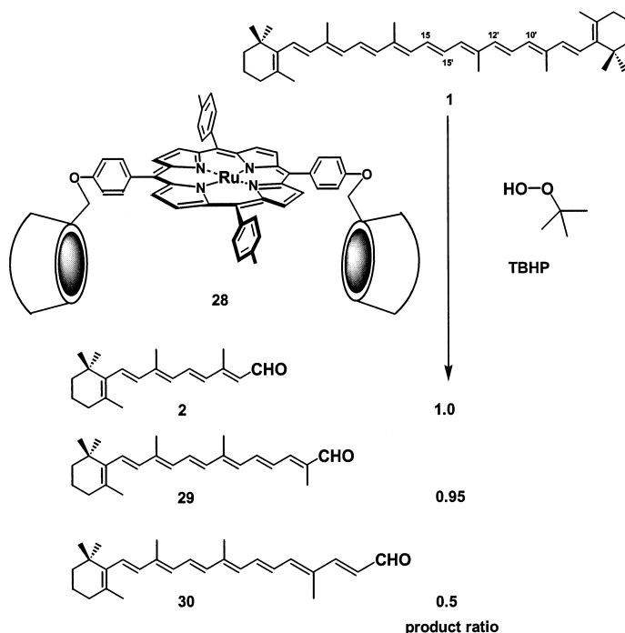
Fig. 11 Cleavage of β-carotene 1 by 28 /TBHP.
